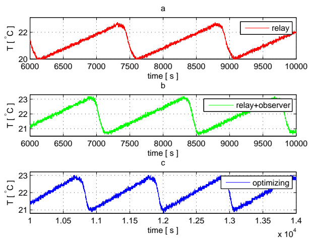
Figure D.9: Comparison: the temperature output from optimizing controller, standard relay controller and relay controller with observer at heating load 500\text{W} . 'optimizing' is the results from the optimizing switch controller. 'relay' refers to experimental results. 'relay+observer' refers to experimental results from a relay controller and observer.
