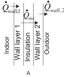
Figure 6.2: wall construction
