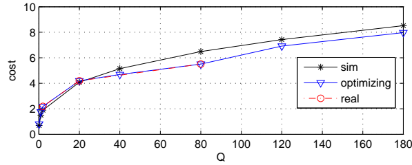
Figure 3.13: Comparison of optimizing switch controller and real optimal solution at heating load 1000W. R is kept at 500. 'sim' is the optimal solution for the model (2.9). 'optimizing' is the optimal solutions by applying the optimizing switch control on the refrigeration system. 'real' is the optimal solution from the pulse experiments with the refrigeration system.
