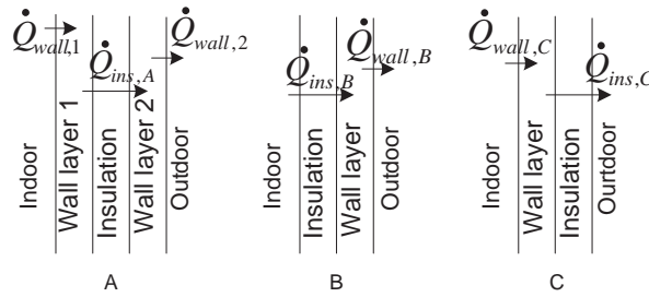
Figure G.3: Different types of wall construction
