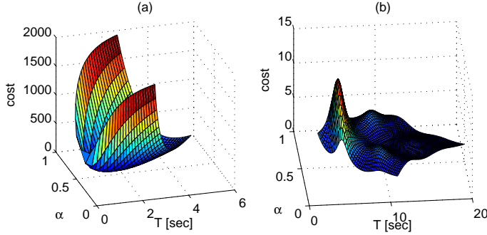
Figure 3.3: Cost J as function of the period T and duty cycle \alpha plotted for second order system \frac{1}{(s-p_1)(s-p_2)} with: (a) poles p_1 = -1, p_2 = -2 , Q = 1, R = 50 . (b) poles p_1 = -0.25 + 1.39i, p_2 = -0.25 - 1.39i , Q = 1, R = 5 .
