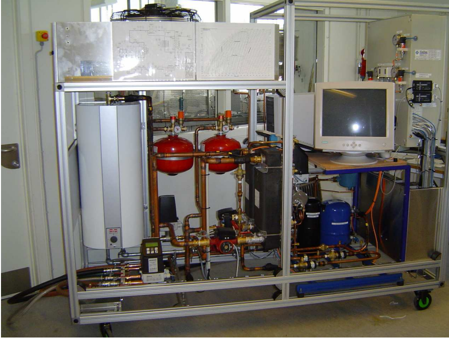
Figure A.11: Refrigeration test plant in Aalborg University
