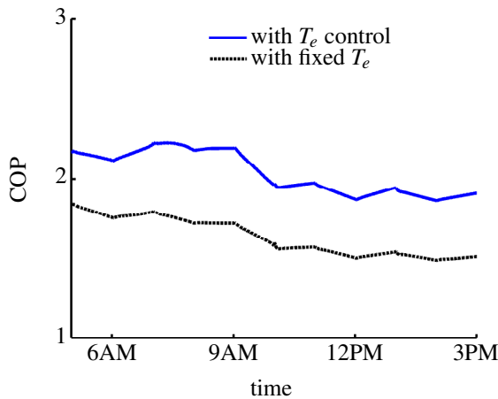
Figure 8.3: A higher COP is achieved by the \hat{T}_e control method.
