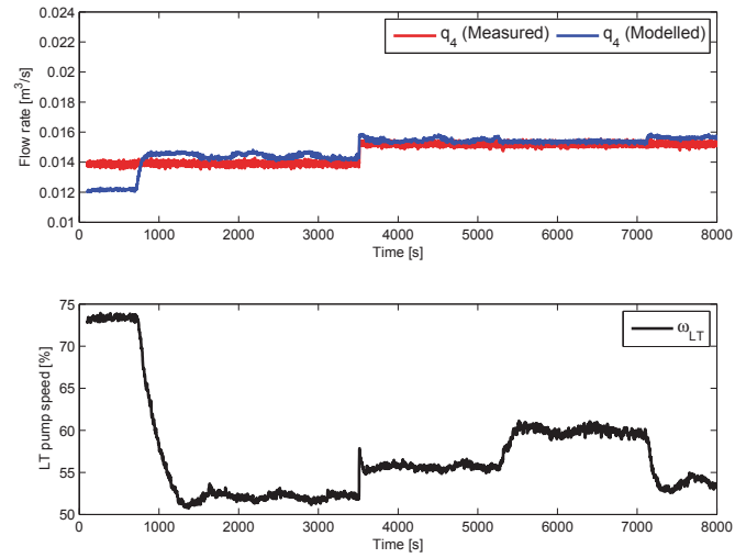
Fig. F.8: Comparison of measured and modeled response for q_4 of the linearized hydraulic model. The deviation for t < 800\text{s} is a result of the linearization of the hydraulic model, and the fact that the system is far from the operating point used for the linearization.
