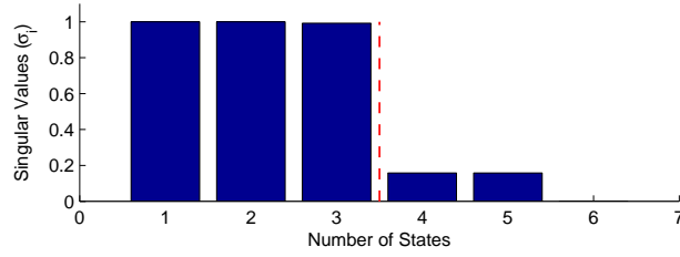
Fig. E.8: Multiplicative-error singular values of H_\infty controller.
