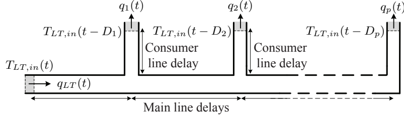
Fig. A.7: The distribution of coolant from the central coolers to the consumers in the LT FW circuit.
