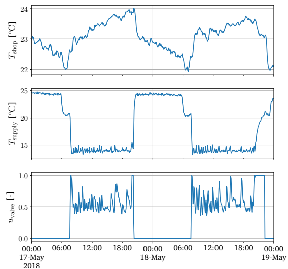
Fig. 3. Initial measurements from the demo-area in Kolding Storcenter. Shop temperature, supply temperature and valve opening for Shop 1 in the demo-area.
