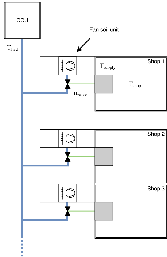
Fig. 1. System layout of demo-area, depicting the three shops and the CCU. Shop 1 is intentionally not adjacent to Shop 2 and Shop 3, as a hallway separates them. The return flow is not depicted in this diagram.
