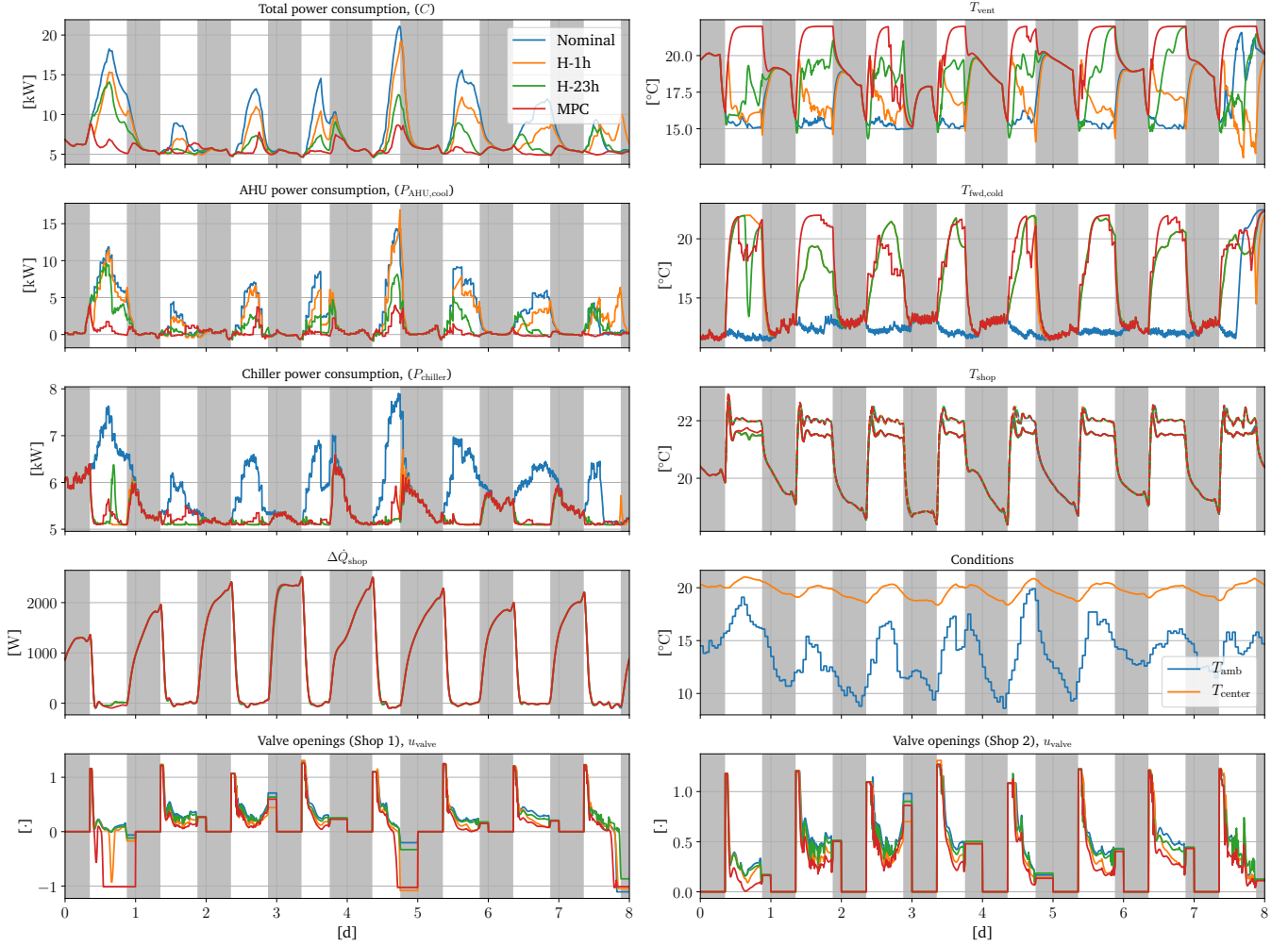
Fig. 6. Simulation results from 8 d simulation, comparison nominal case to three different control strategies. Shaded area indicates no control authority. Shop temperature, T_{\text{shop}} is depicted as a solid line for Shop 1 and a dashed line for Shop 2 . Valve opening signals, u_{\text{valve}} , combines signal for both heating valve ( > 0 ) and cooling valve ( < 0 ).
